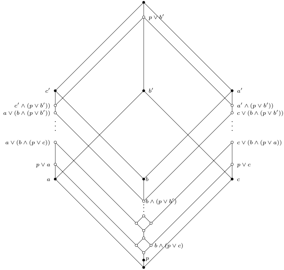
FIGURE 9. The free lattice generated by \mathbf{B}_3 and p , 0 \leq p \leq b .
