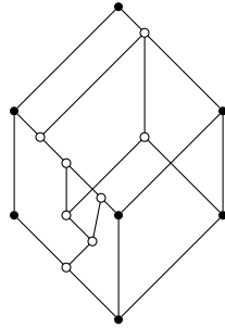
FIGURE 5. The largest minimal extension of \mathbf{D}_1
