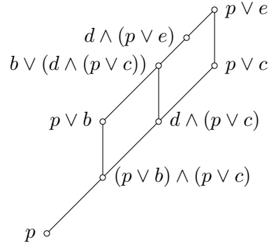
FIGURE 4. S
