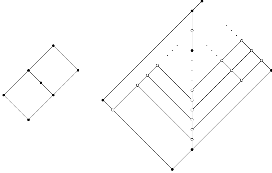
FIGURE 22. \mathbf{G}_7 and an infinite minimal extension.
