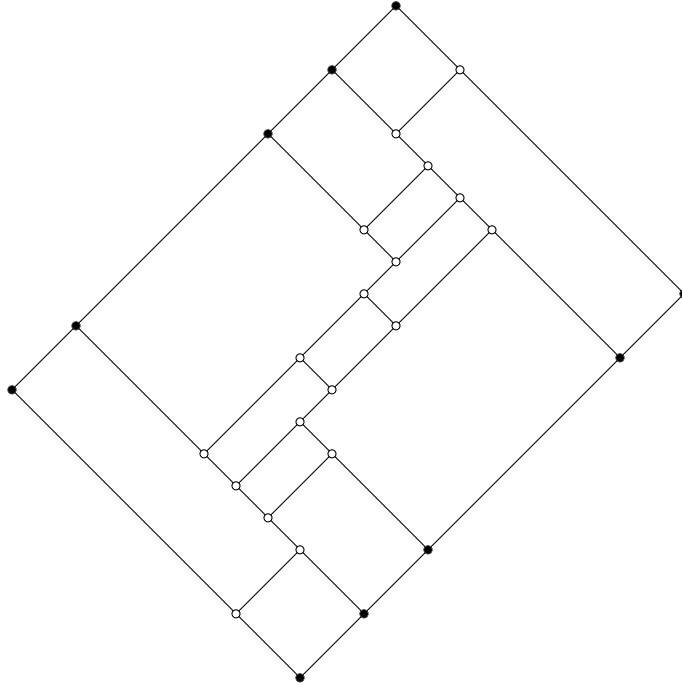
FIGURE 11. The largest minimal extension of \mathbf{2} \times \mathbf{5} .
