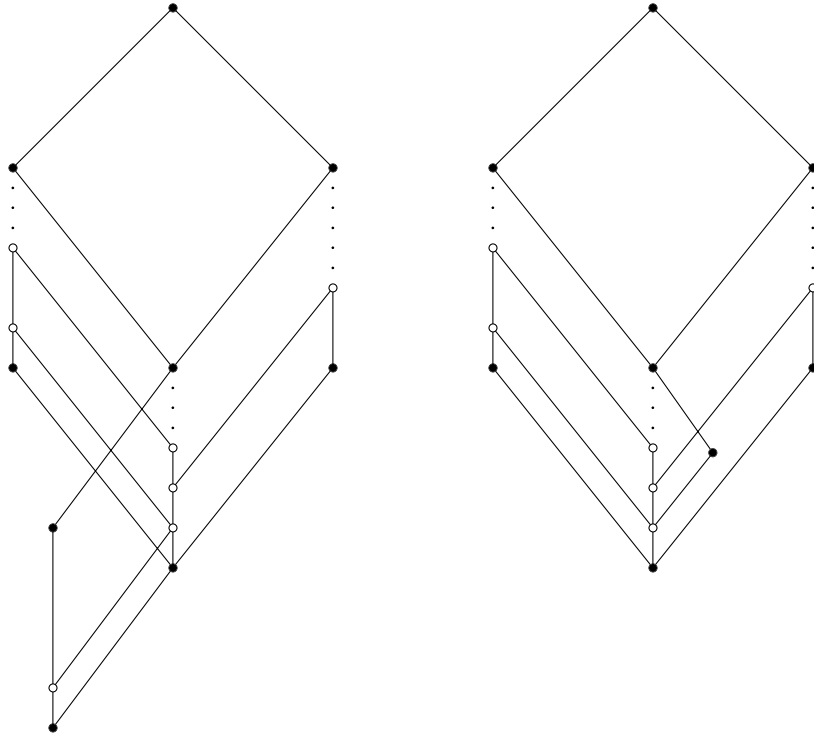
FIGURE 18. Minimal extensions of \mathbf{G}_{13} and \mathbf{G}_9 .
