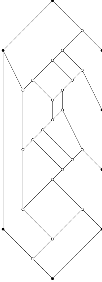
FIGURE 14. The largest minimal extension of \mathbf{N}_{24} .
