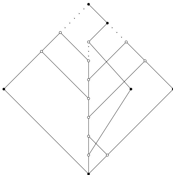
FIGURE 21. An infinite minimal extension of \mathbf{G}_6 .
